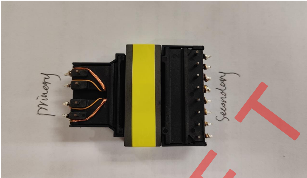
Fig. 16: External view-2 of transformer T101
