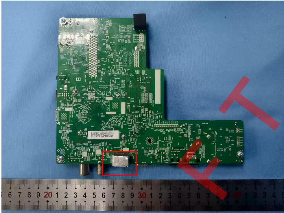
Fig. 12: Soldering side view_1 of main board for configuration A
