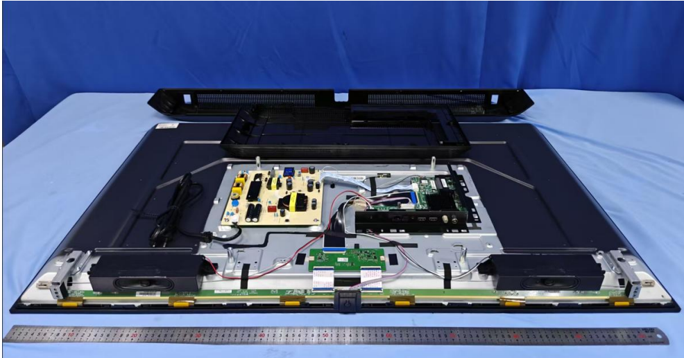
Fig. 4: Internal view-2 of the equipment for configuration A (configuration 1)
