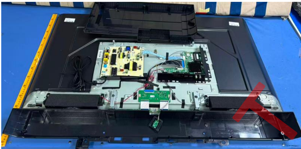
Fig. 22: Internal view_1 of equipment
