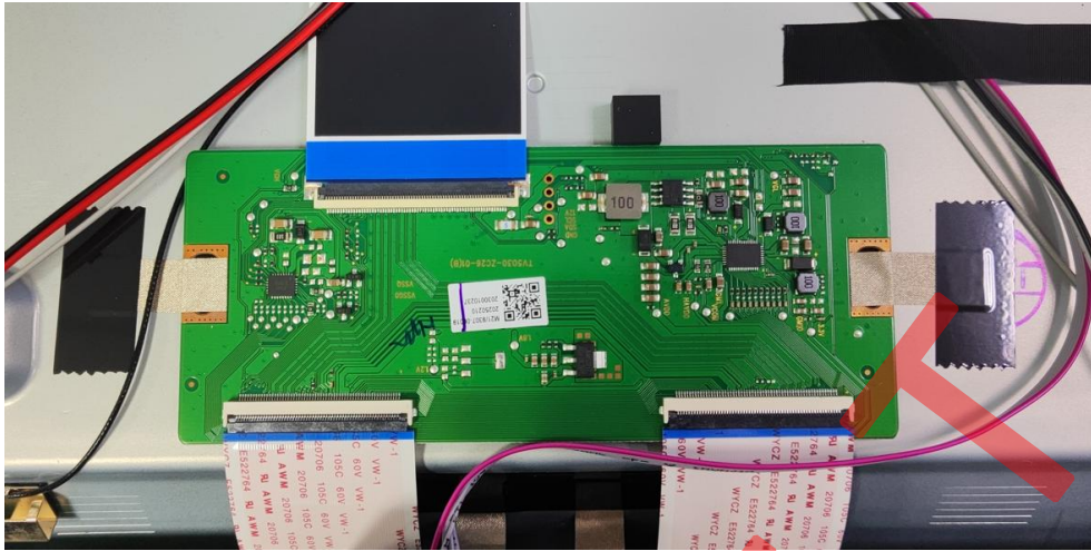
Fig. 14: Component side view of control board
