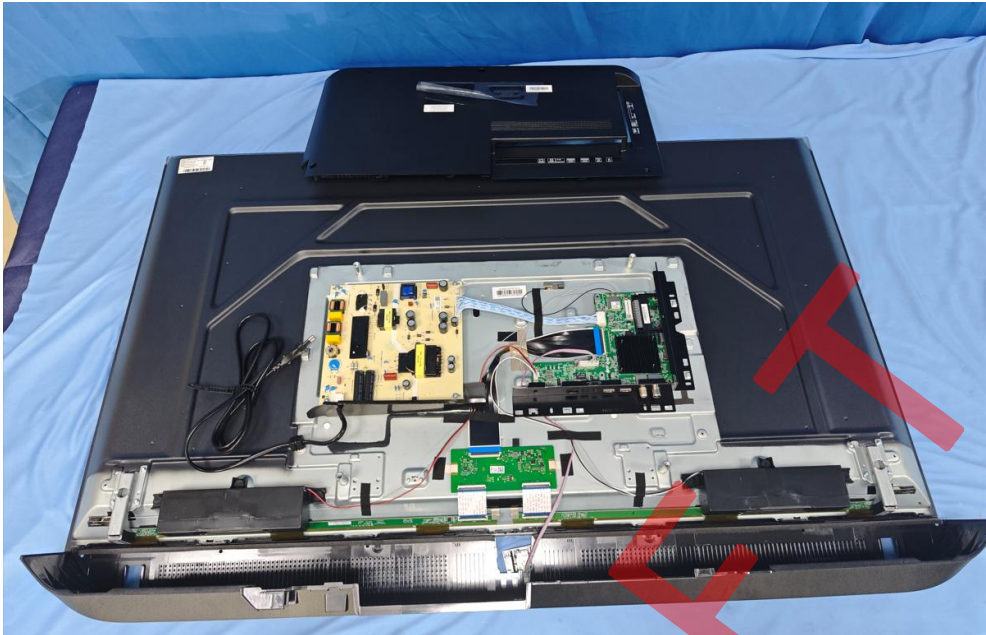
Fig. 3: Internal view-1 of the equipment for configuration A (configuration 1)
