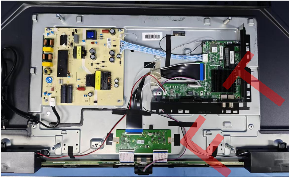
Fig. 6: Internal view-4 of the equipment for configuration A (configuration 2)
