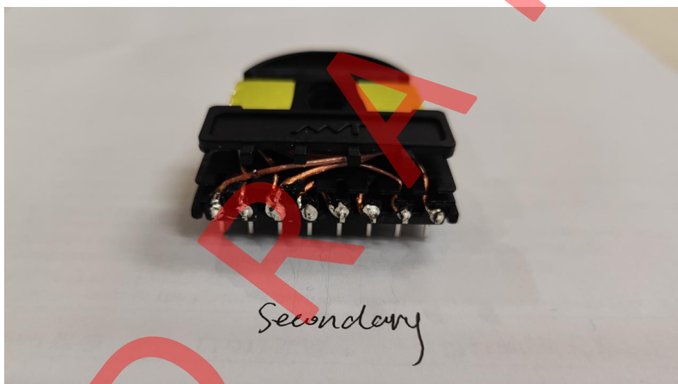
Fig. 19: Internal view-3 of transformer T101
